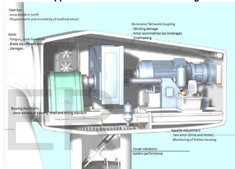
Fig.6.1 Applications of condition monitoring in wind turbine
