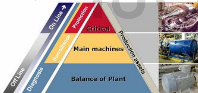
Fig.1.2 Different approaches to condition based maintenance for different equipment in plant
